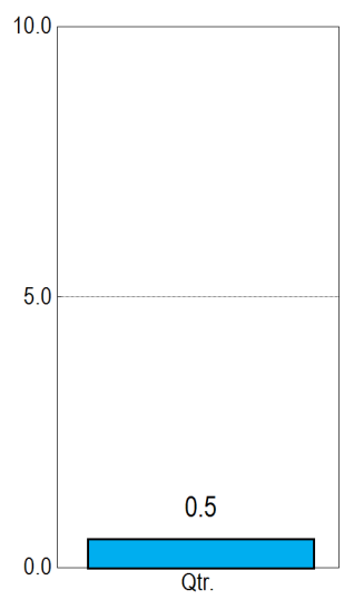
Information Ratio
